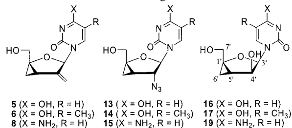
Figure 1. C-4'-modified pyrimidine nucleosides built on a 2-oxabicyclo[3.1.0]hexane scaffold. Numbering used as shown for 16–19 .
