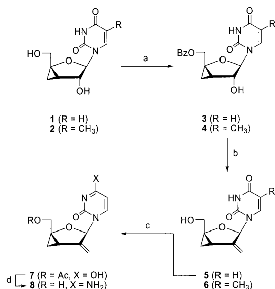
Scheme 1. a) BzCl, DMF, pyridine, 0 °C; b) i. periodinane, CH 2 Cl 2 , 0 °C; ii. C 2 H 5 C(CH 3 ) 2 ONa, PPh 3 MeBr, THF; iii. MeOH, MeONa; c) Ac 2 O, pyridine; d) i. Lawesson's reagent, 1,2-dichloroethane, reflux; ii. MeOH/NH 3 .
