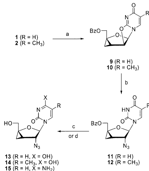
Scheme 2. a) i. DEAD, PPh 3 , BzOH, DMF; ii. DEAD, PPh 3 ; b) NaN 3 , 18-crown-6, DMF, reflux; c) MeOH, MeONa; d) i. 1,2,4-triazole, pyridine, 4-chlorophenyl phosphorodichloridate; ii. NH 4 OH, dioxane; iii. MeOH, MeONa.
