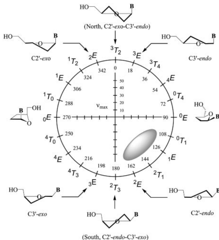
Figure 2. Pseudorotation cycle for nucleosides showing the characteristic North, South, East and West conformations. The units of P and v_{\max} values are degrees. Envelope ( E ) and twist ( T ) forms alternate every 18°. The shaded area indicates the preferred pseudorotational region for nucleosides 2 , 6 , 14 and 17 .
