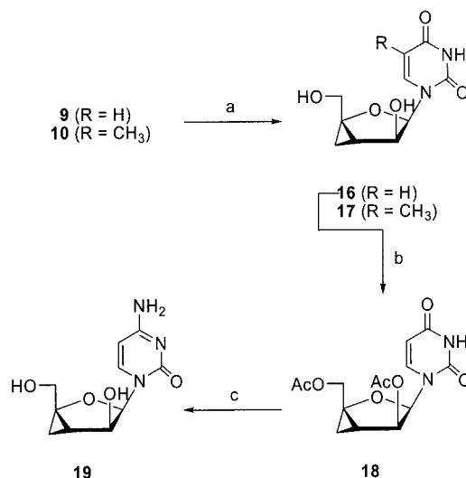
Scheme 3. a) 1 N NaOH, MeOH; b) Ac 2 O, pyridine; c) i. Lawesson's reagent, 1,2-dichloroethane, reflux; ii. MeOH/NH 3 , 100 °C.
